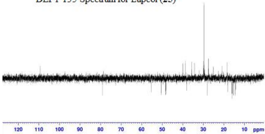
DEPT 135 Spectrum for Lupeol (25)
