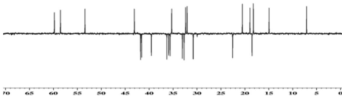
DEPT 135 Spectrum for Friedelin (133)
