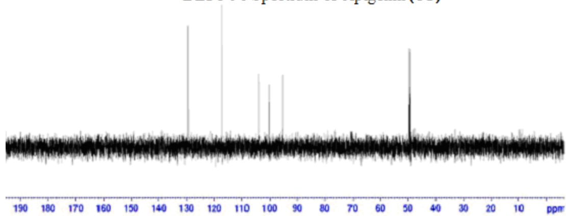
DEPT 90 Spectrum of Apigenin (68)
