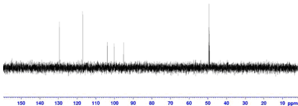
DEPT 135 Spectrum for Apigenin (68)
