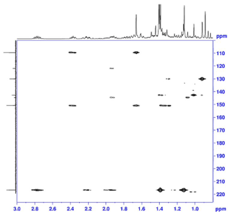
HMBC Spectrum of Lupenone (135)
