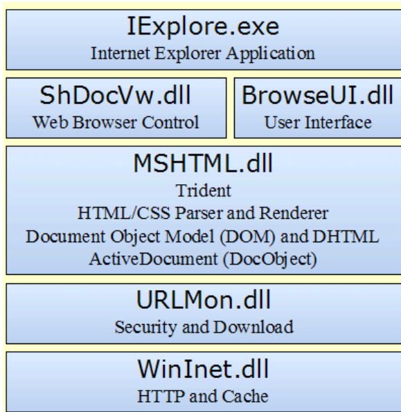
Figure 3.2: Internet Explorer Architecture
