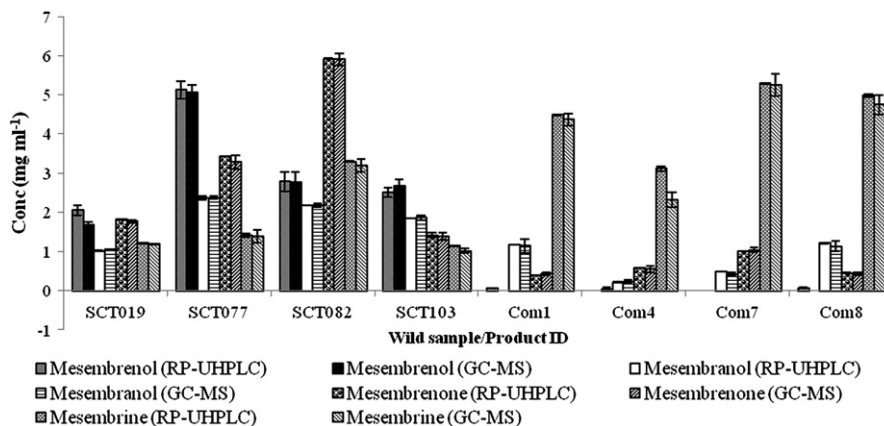
Fig. 4. Quantitative data for alkaloids in raw materials and products as determined by RP-UHPLC PDA and GC-MS analyses.
